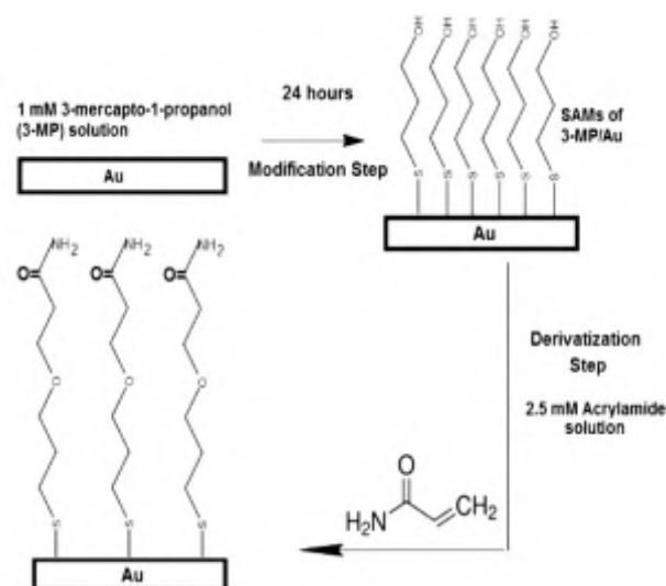
Scheme 1. Complete process of modification and reaction on gold surfaces.
