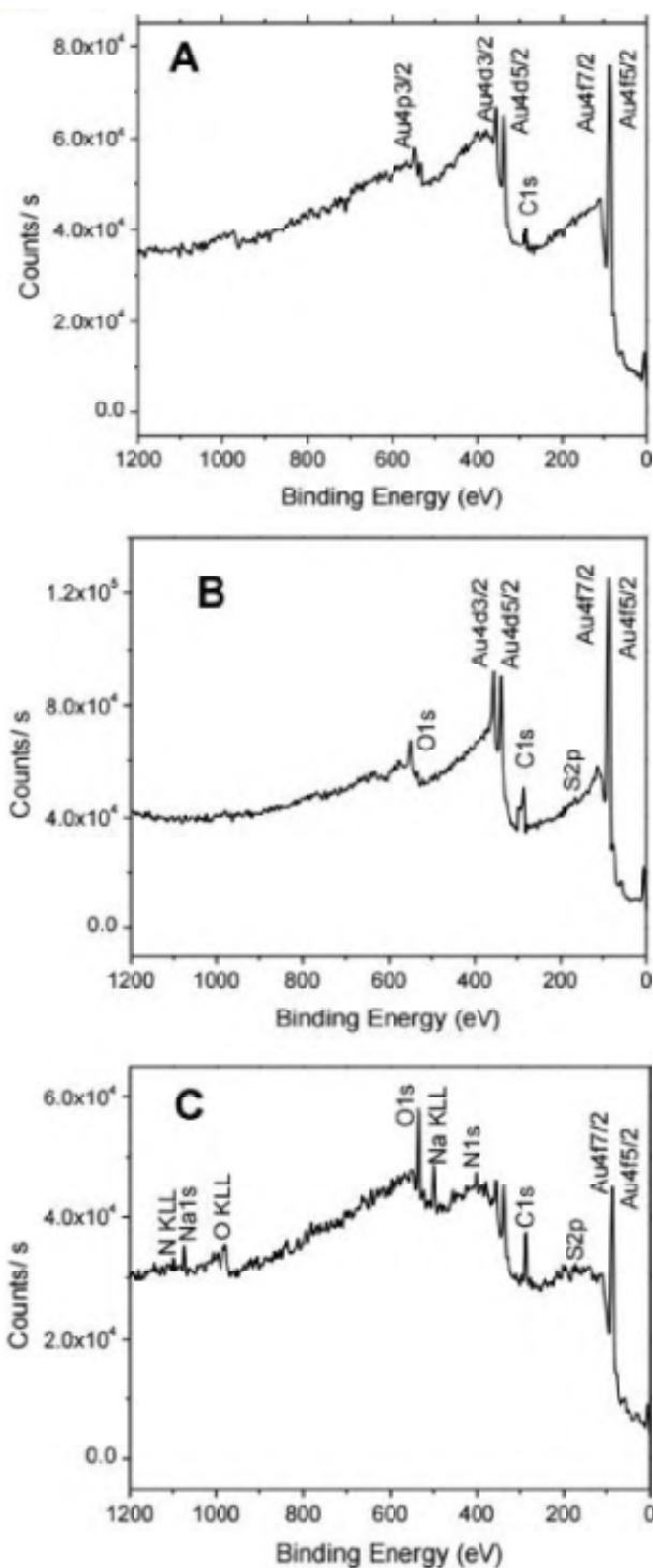
Figure 3. XPS spectra of the (A) bare Au, (B) 3-MP/Au, and (C) AA/3-MP/Au electrode systems.
